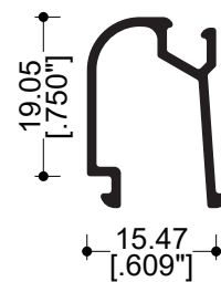
012576 Junquillo colonial
