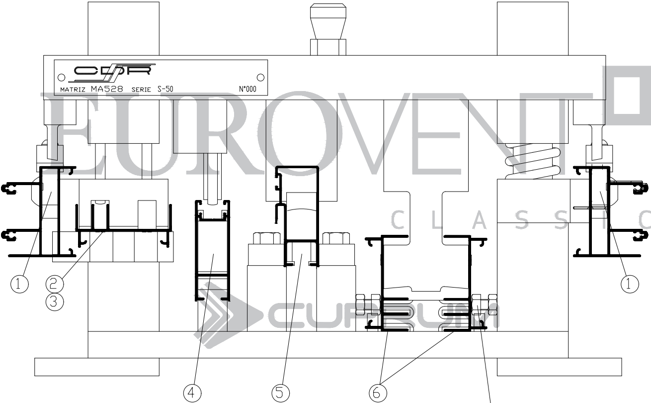
VISTA FRONTAL
