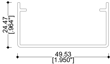
GN-196 Canal "U" PVC
