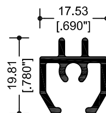
63727 BARROTILLO 2"
