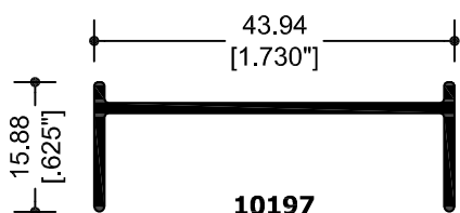
10197 JAMBA LATERAL
