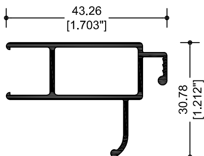
7112 VERTICAL MOSQUITERO
