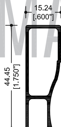
9756 MARCO 1 1/4"
