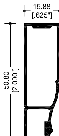
10103 MARCO 2"
