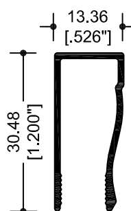
13563 MARCO 1 1/4"
