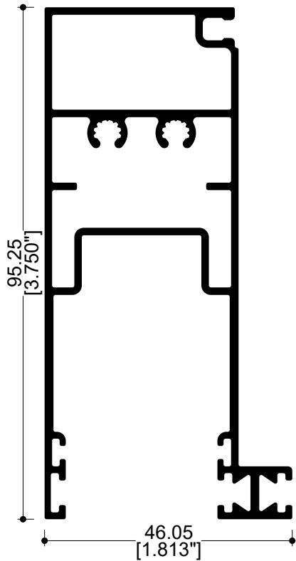
70949 Zoclo mosquitero
