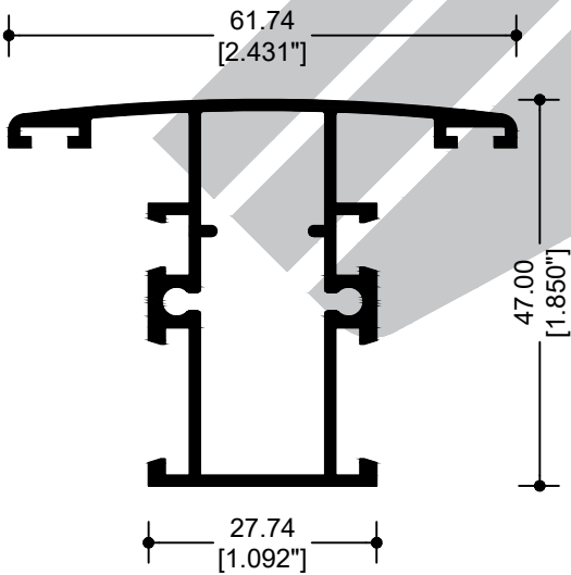
62028 "T" INTERMEDIO
