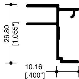
68847 EXTENSION JAMBA
