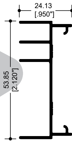
68844 JAMBA
