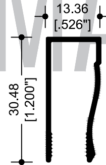
13563 MARCO 1 1/4"
