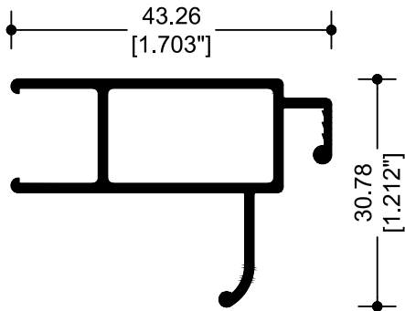
7112 VERTICAL MOSQUITERO
