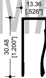
13563 MARCO 1 1/4"
