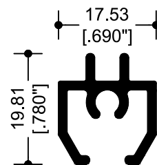
63727 BARROTILLO 2"
