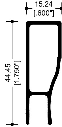
9756 MARCO 1 3/4"
