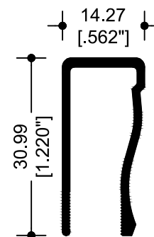
9525 MARCO 1 1/4"
